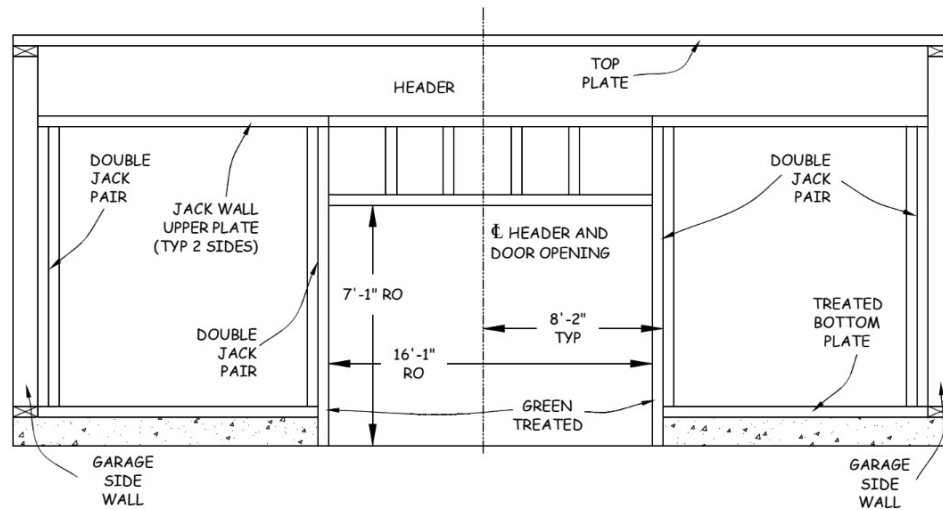
Figure 23.4. Overhead Door (OHD) Wall Assembly.
