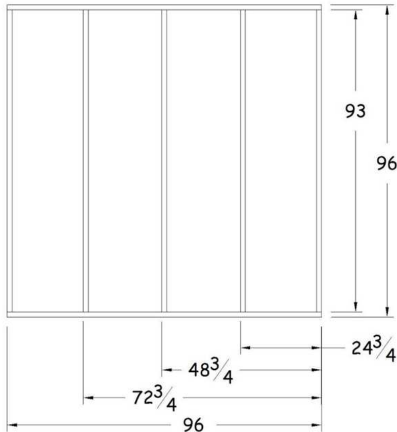
Figure 22-1. Floor Framing.
