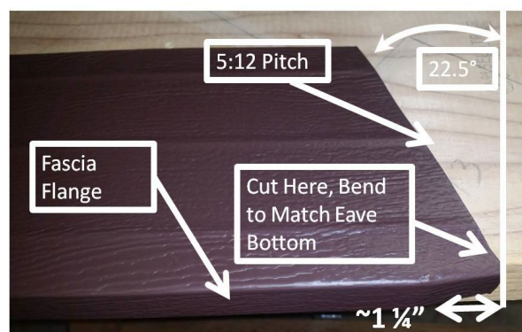
Figure 11-26. Eave End Gable Fascia.
