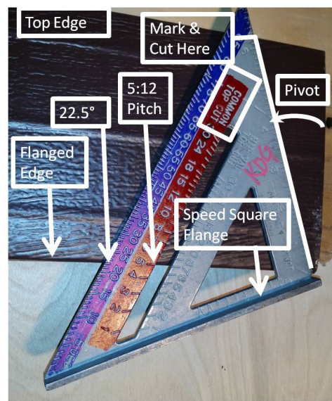
Figure 11-25. Marking Gable Eave End Fascia Angle.
