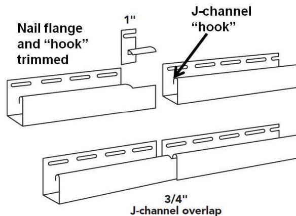
Figure 11-7. J-Channel Splice.
