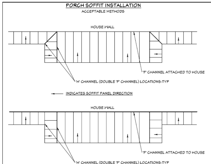
Figure 11-23. Porch Soffit.
