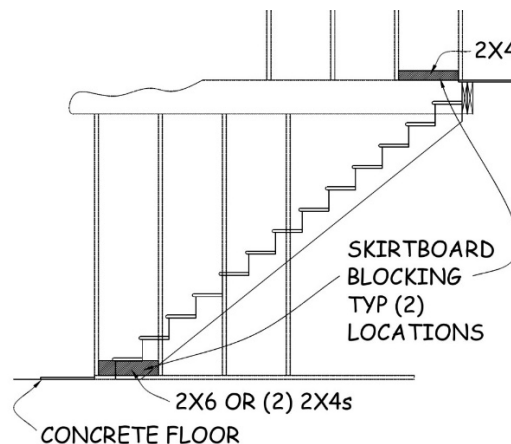
Figure 10-7. Blocking for Skirtboard.
