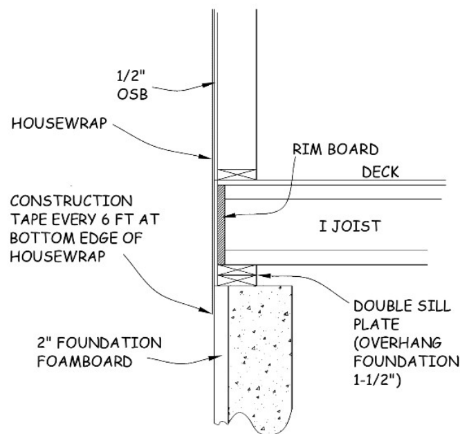
Figure 5-3. Sill Box with OSB and House Wrap.
