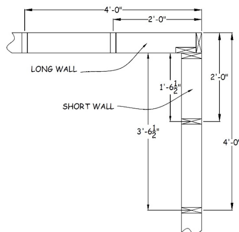
Figure 3-4. Corner Layout.
