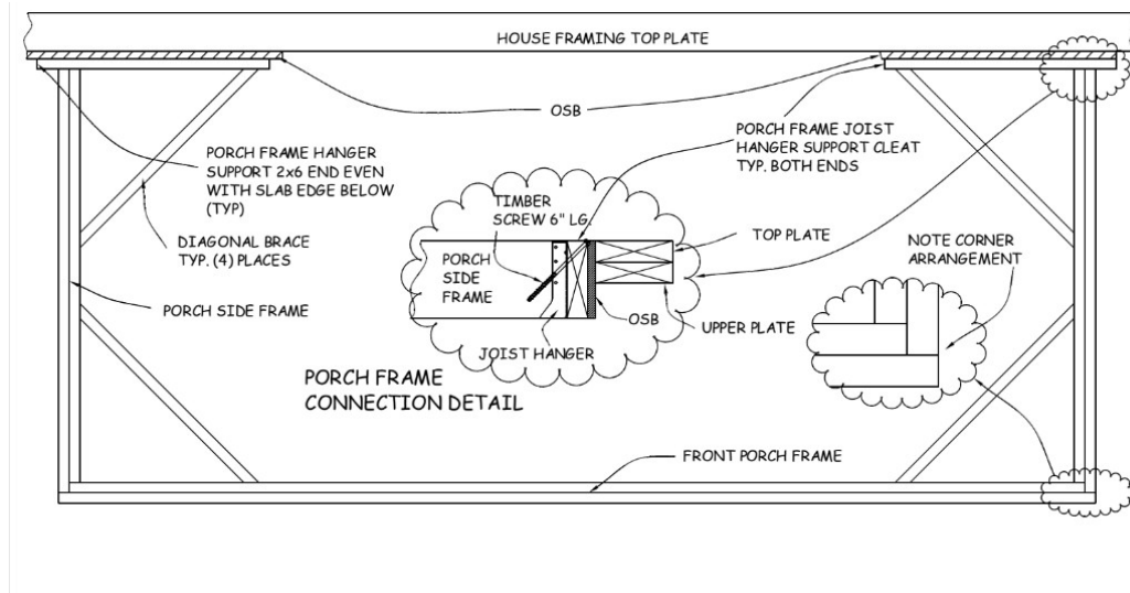
Figure 6-4. Porch Framing.
