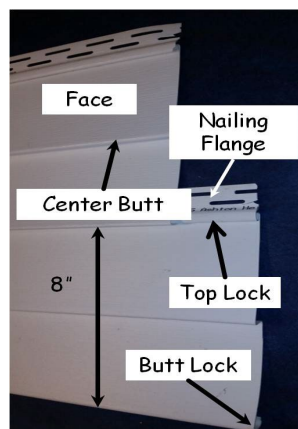
Figure 11-21. Siding Nomenclature.
