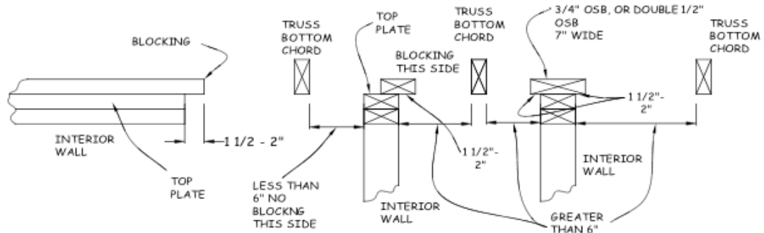
Figure 10-4. Blocking For Ceiling Rock.
